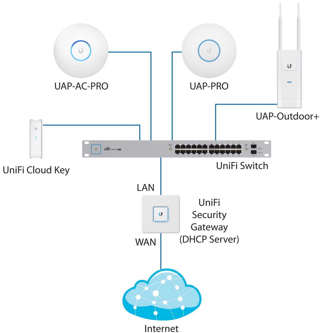
Sample Network Diagram
