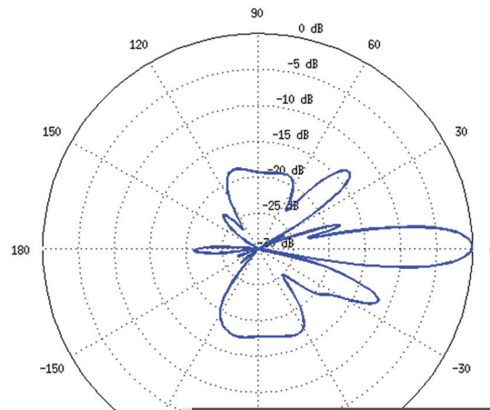
Horizontal Elevation
